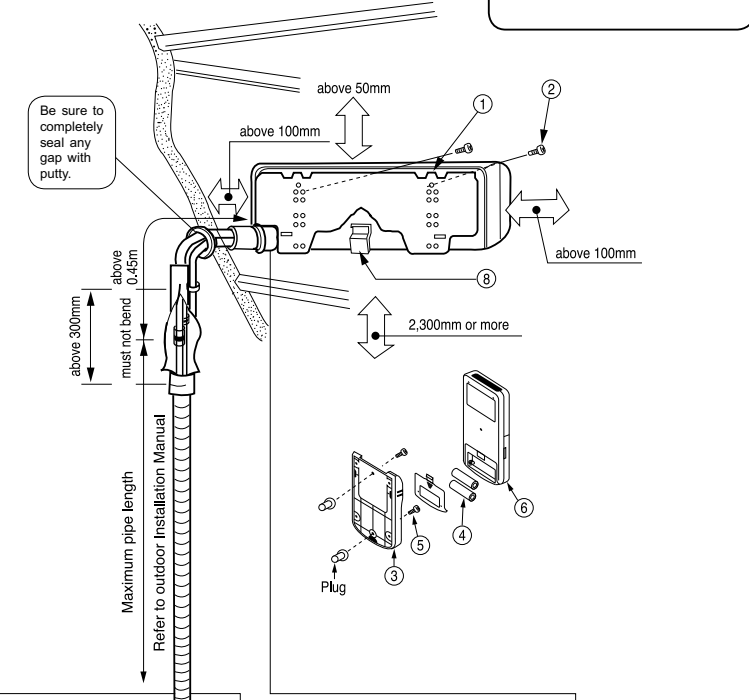
Figure showing the Installation of Indoor Unit.
