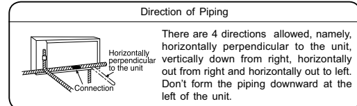
Figure showing the Installation of Indoor Unit.
