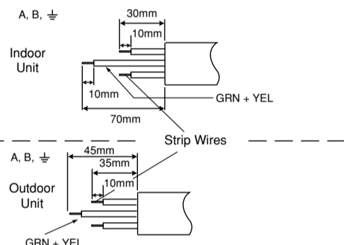
Detail of cutting the connecting cord
